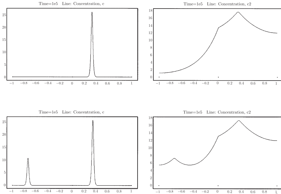
Figure 5. Long-time limit of the solution to (1.1)–(1.3) with \epsilon^2 = 0.0001 and D(x) = 0.1 for -1 < x < 0 , D(x) = 0.5 for 0 < x < 1 . We observe an interior spike on the right subinterval or two interior spikes on different subintervals, respectively.
