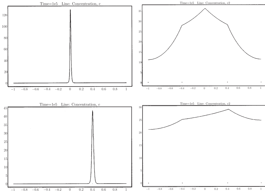
Figure 3. Long-time limit of the solution to (1.1)–(1.3) with \epsilon^2 = 0.0001 and D(x) = 1 for -1 < x < -0.4 , 0.4 < x < 1 , D(x) = 5 for -0.4 < x < 0.4 . We observe an interior spike in the central interval and a spike near a jump.
