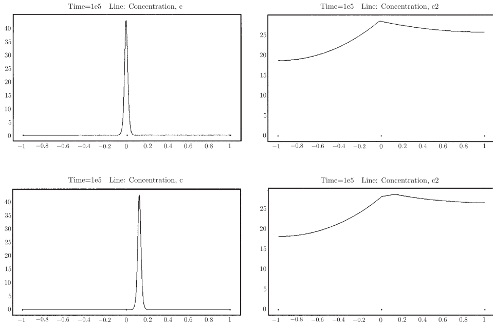
Figure 1. Long-time limit of the solution to (1.1)–(1.3) with \epsilon^2 = 0.0001 and D(x) = 1 for -1 < x < 0 , D(x) = 5 for 0 < x < 1 . We observe a spike near the jump discontinuity of the inhibitor diffusivity and a spike in the right subinterval, respectively. The conditions (3.1) and (3.5), respectively, are satisfied.
