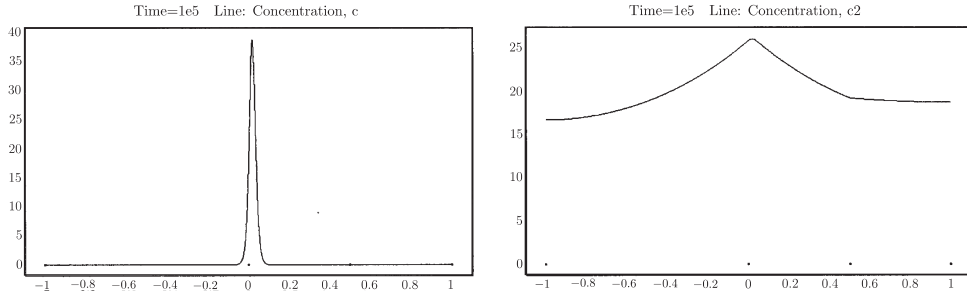
Figure 2. Long-time limit of the solution to (1.1)–(1.3) with \epsilon^2 = 0.0001 and D(x) = 1 for -1 < x < 0.5 , D(x) = 5 for 0.5 < x < 1 . We observe an interior spike in the left subinterval. The condition (3.5) is satisfied.
