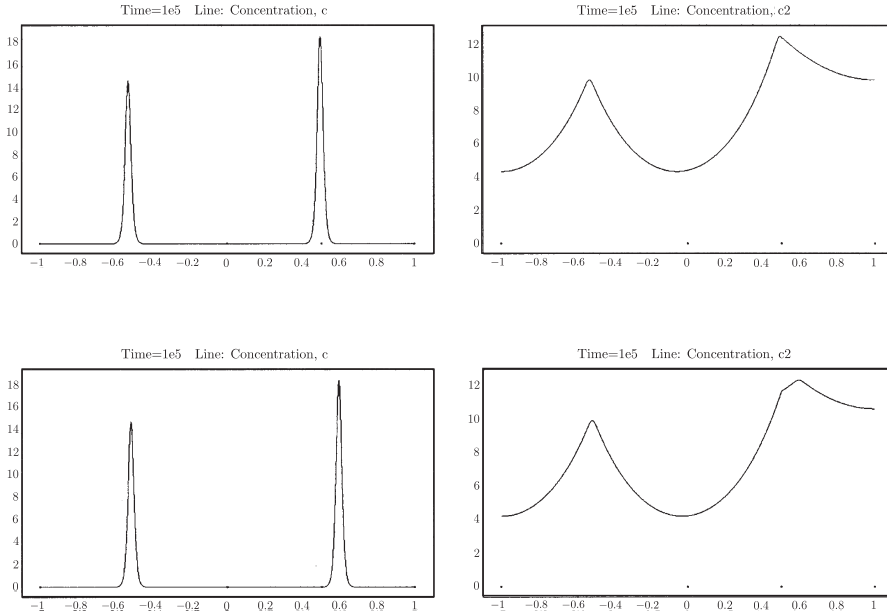
Figure 6. Long-time limit of the solution to (1.1)–(1.3) with \epsilon^2 = 0.0001 and D(x) = 0.1 for -1 < x < 0.5 , D(x) = 0.5 for 0.5 < x < 1 . We observe an interior spike in the left subinterval and a spike near the jump discontinuity or two interior spikes on different subintervals, respectively.
