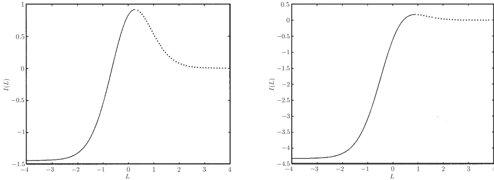
Figure B. The left and right figures corresponds to I(L) for \beta = 0.2 and \beta = 0.6 , with maximum values about 0.92 and 0.17, located at about 0.26 and 0.90 respectively. As will be shown in the next section, the dotted lines and solid lines corresponds to unstable and stable steady states respectively.
