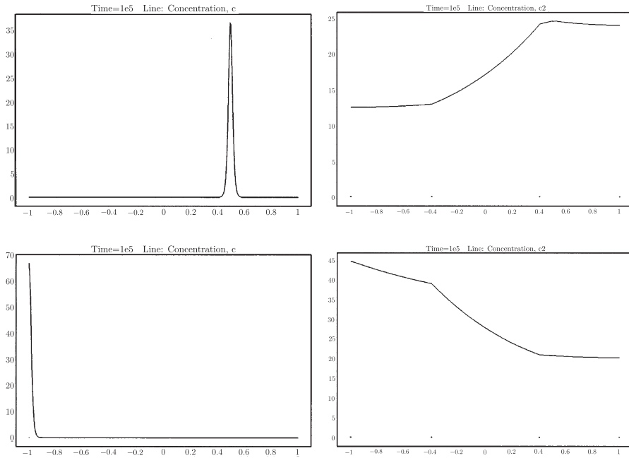
Figure 4. Long-time limit of the solution to (1.1)–(1.3) with \epsilon^2 = 0.0001 and D(x) = 5 for -1 < x < -0.4 , 0.4 < x < 1 , D(x) = 1 for -0.4 < x < 0.4 . We observe an interior spike in the right interval and a boundary spike.
