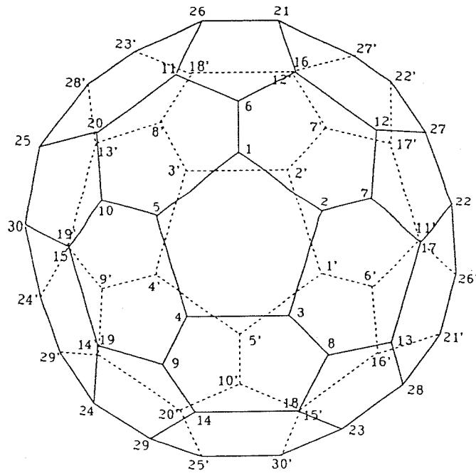
Figure 9. Labeling of the Buckminsterfullerene C_{60} .
