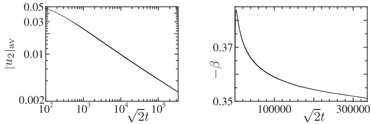
(g) |u_2|_{av} ( \sqrt{2}t \leq 336000 )
