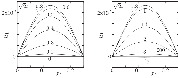
(e) u_1 ( \sqrt{2}t \leq 200 )
