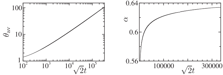
(f) \theta_{av} ( \sqrt{2}t \leq 336000 )
