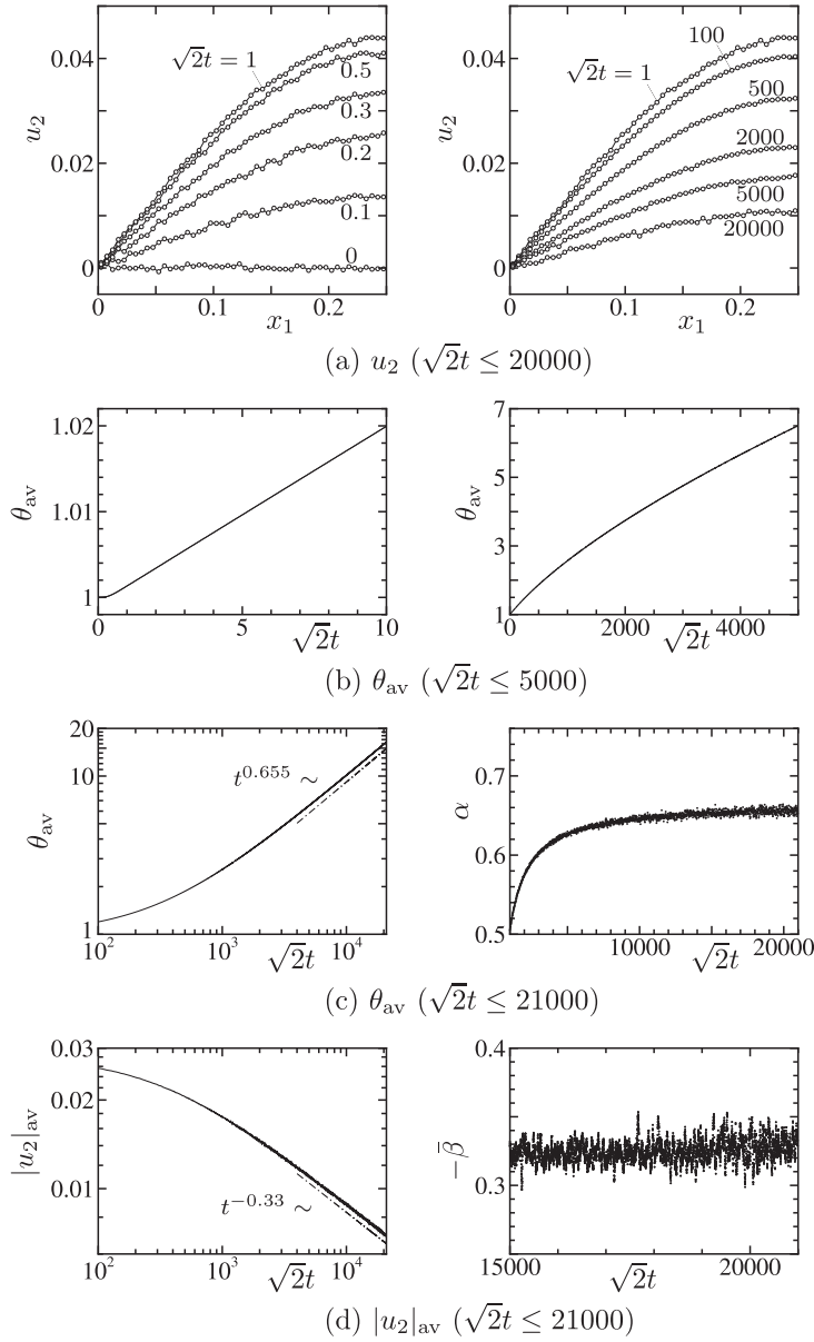
Figure 4.4: Boltzmann equation with \text{Kn} = 0.1 and f_0 = 0.2 . The result shown here is based on the ensemble average over N independent runs and time average over the interval [t - C/\sqrt{2}, t + C/\sqrt{2}] , where N and C are chosen appropriately depending on t . The details are given in the main text. The \bar{\beta} is the average of \beta over the time interval [t - 10000/\sqrt{2}, t] .
