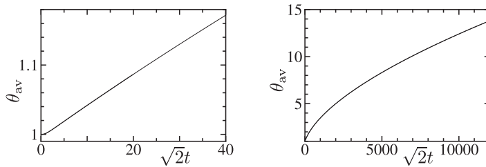
(b) \theta_{av} ( \sqrt{2}t \leq 12000 )
