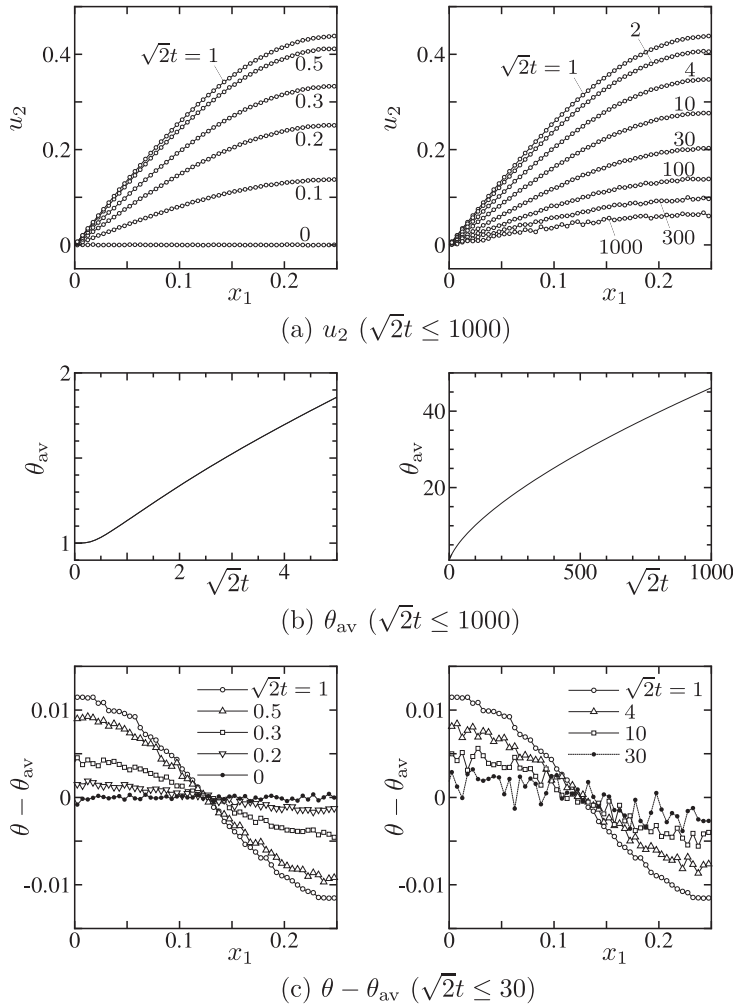
Figure 4.3: Boltzmann equation with \text{Kn} = 0.1 and f_0 = 2 . The ensemble average over 96 independent runs is shown. The \bar{\beta}(t) is the time average of \beta over the interval [t - 500/\sqrt{2}, t] .
