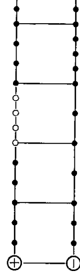
Figure 15. Here the equal-distance portion is transient.
