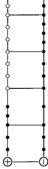
Figure 14. A zigzagging chain and its vertices.
