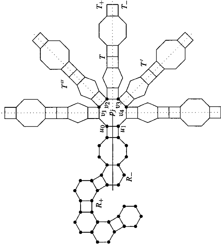
Figure 6. During the process of straightening!
