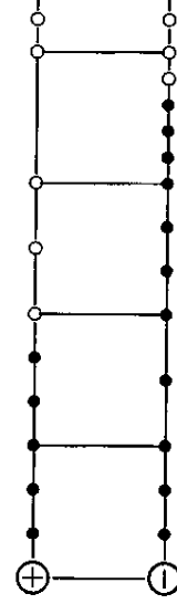
Figure 16. Here most vertices are equidistant to the ends.
