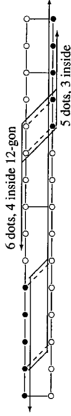
Figure 19. The straightened chain.
