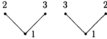
FIGURE 2. Two ordered trees.
