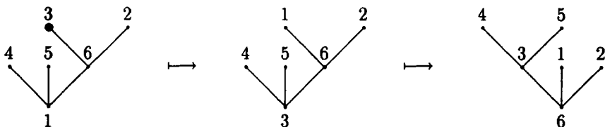
FIGURE 5. The bijection with l = 3 and r = 6 .
