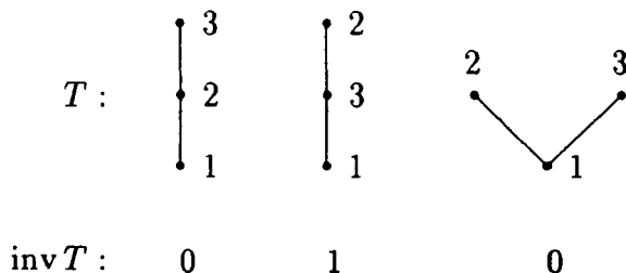
FIGURE 1. Trees and inversions for n = 3 .
